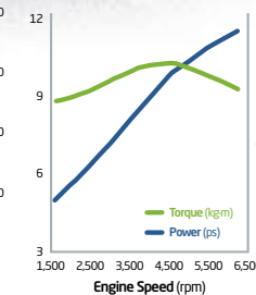
KAPPA 1.0 FFV ENGINE
